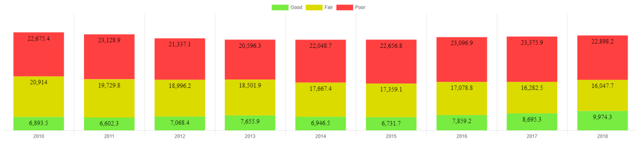
Pavement Condition Trends State - Agencies with 100+ Centerline Miles, County Road Commission, Federal Aid Lane Miles
