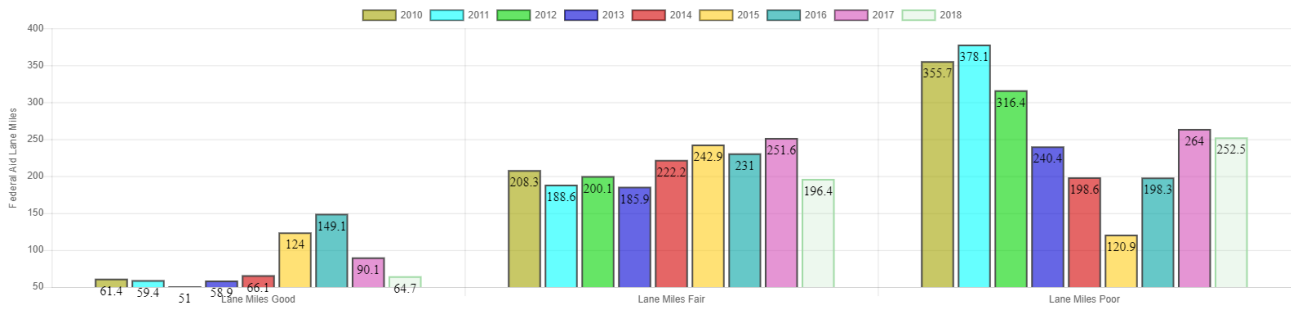
Pavement Condition Trends County - St. Joseph, County Road Commission, Federal Aid Lane Miles
